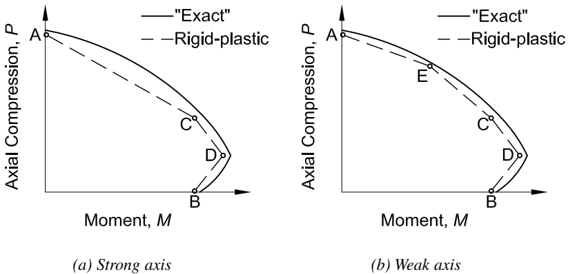
Fig. C-II.1. Comparison between exact and simplified moment-axial compressive force cross-section strength envelopes.
