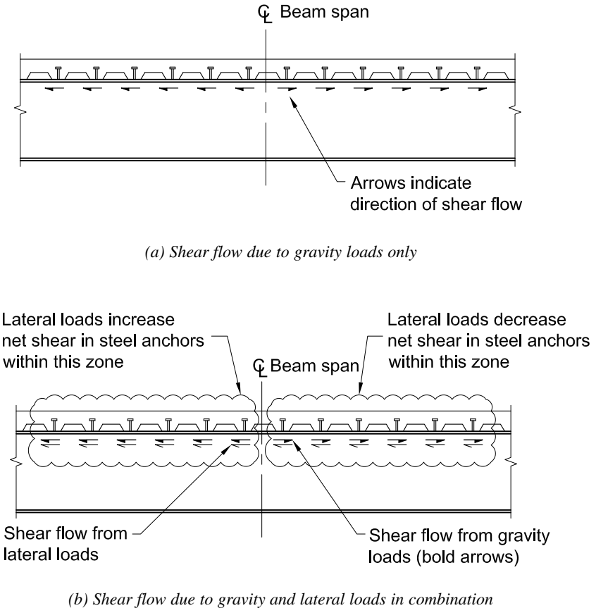
Fig. C-17.1. Shear flow at collector beams.
